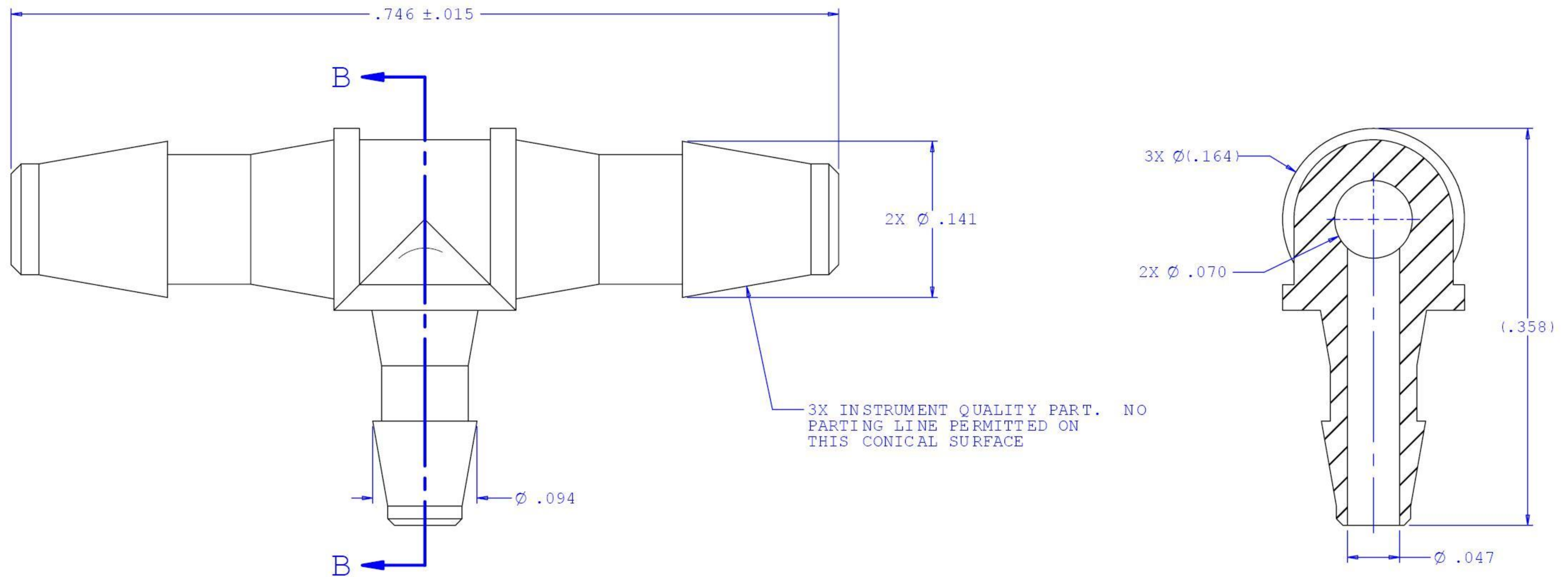
SECTION B-B
