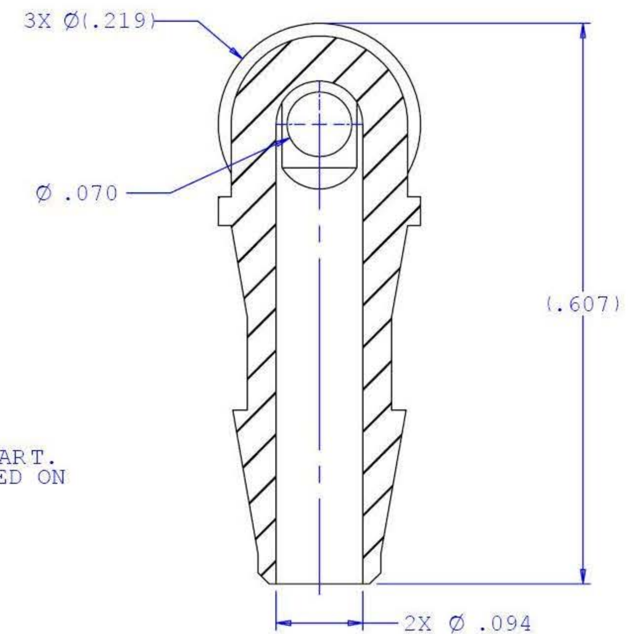
SECTION B-B
