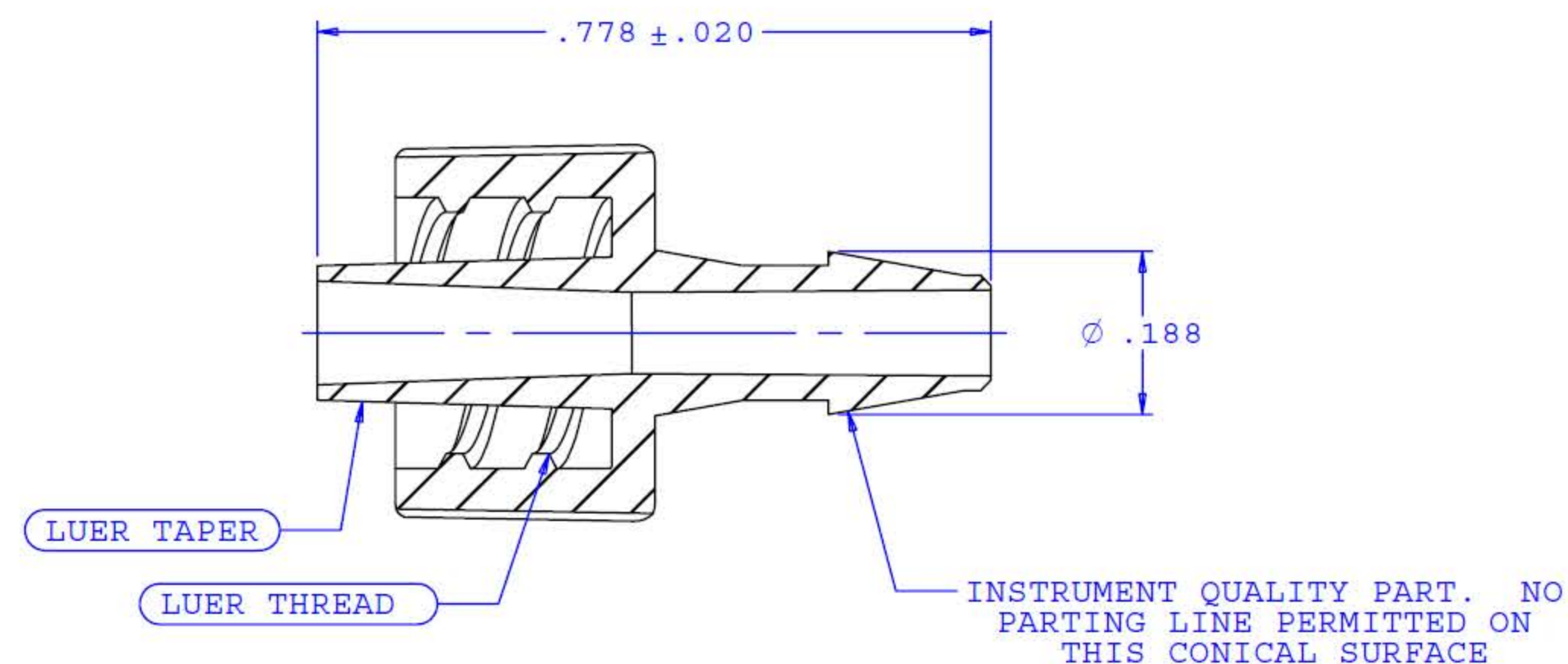
SECTION B-B
