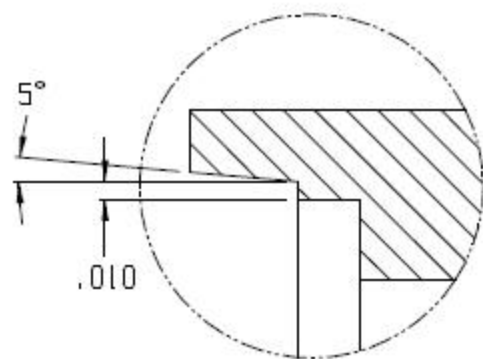
DETAIL B SCALE 10:1 4 LEGS
